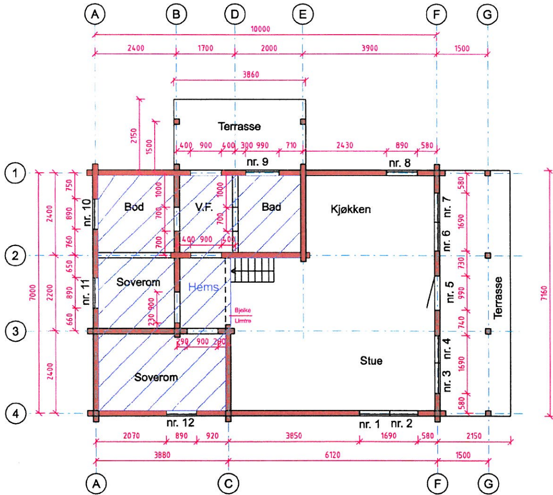
Plan 1 etg
